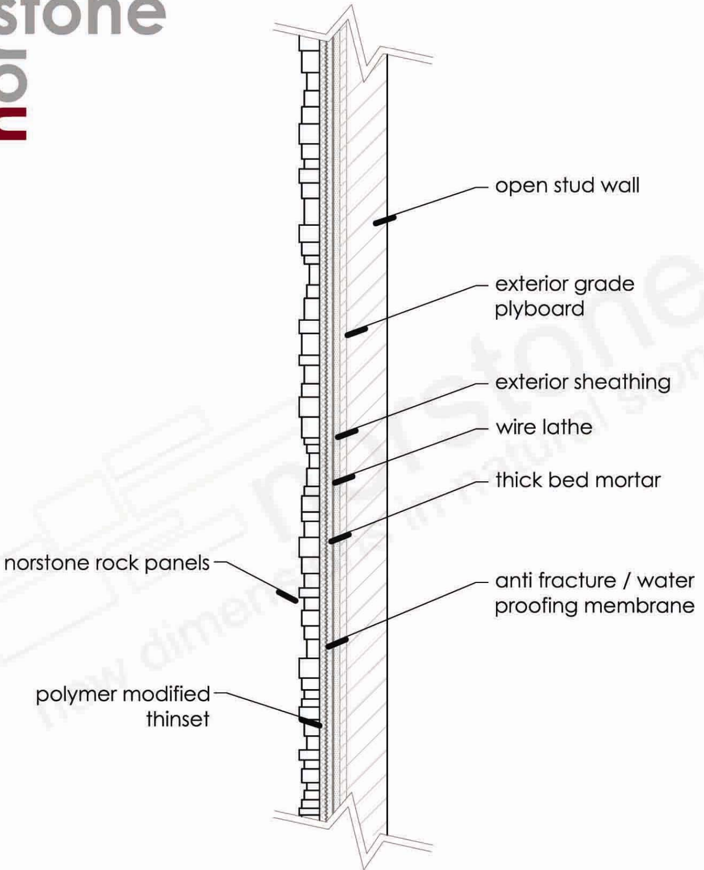
rock panel detail - open stud wall - exterior #2
